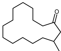
Cyclopentadecanone, 3-methyl-
